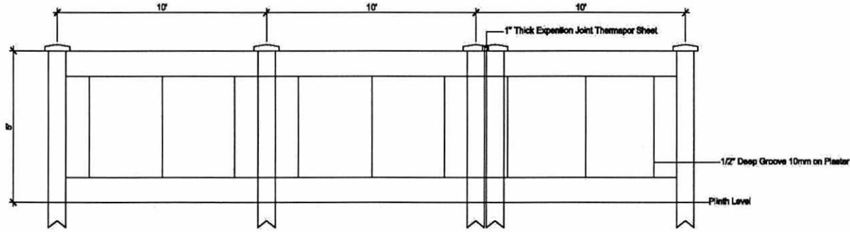
3/4" Cement Plaster Boundary Wall Detail Inner & Outer Side
