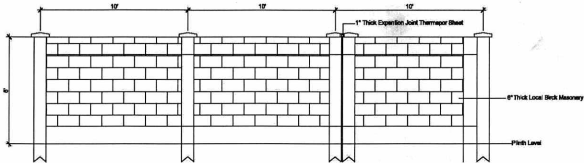
Block Masonry Boundary Wall Detail
