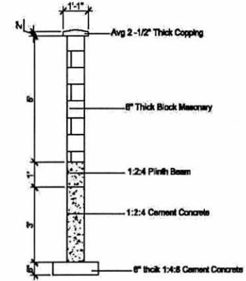
Situ & Wall Detail
