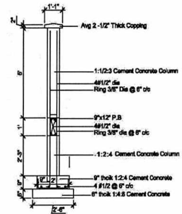
Column Footing Detail
