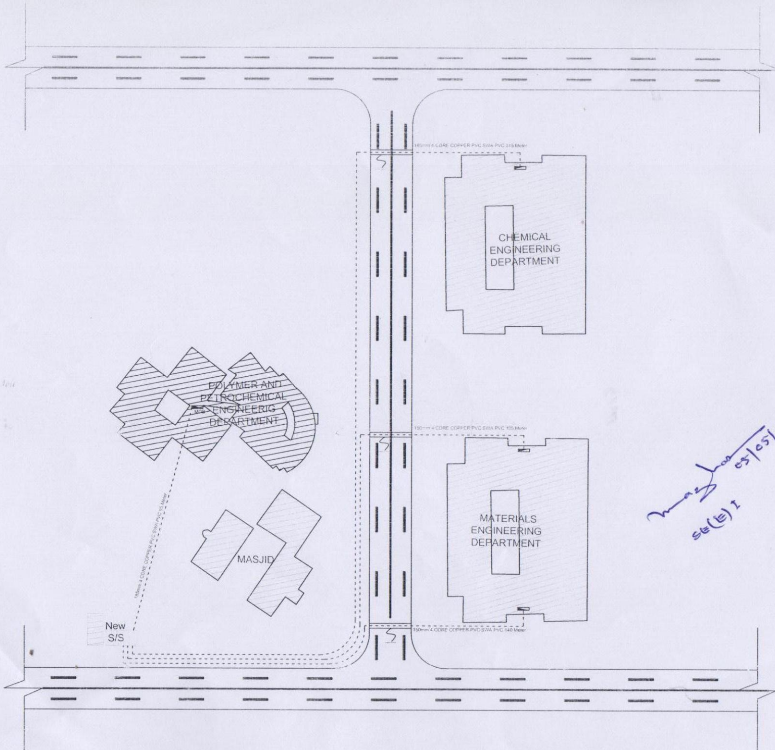
CABLE ROUTE FOR CHEMICAL, MATERIAL, POLYMER AND PETROCHEMICAL ENGINEERING DEPARTMENT
