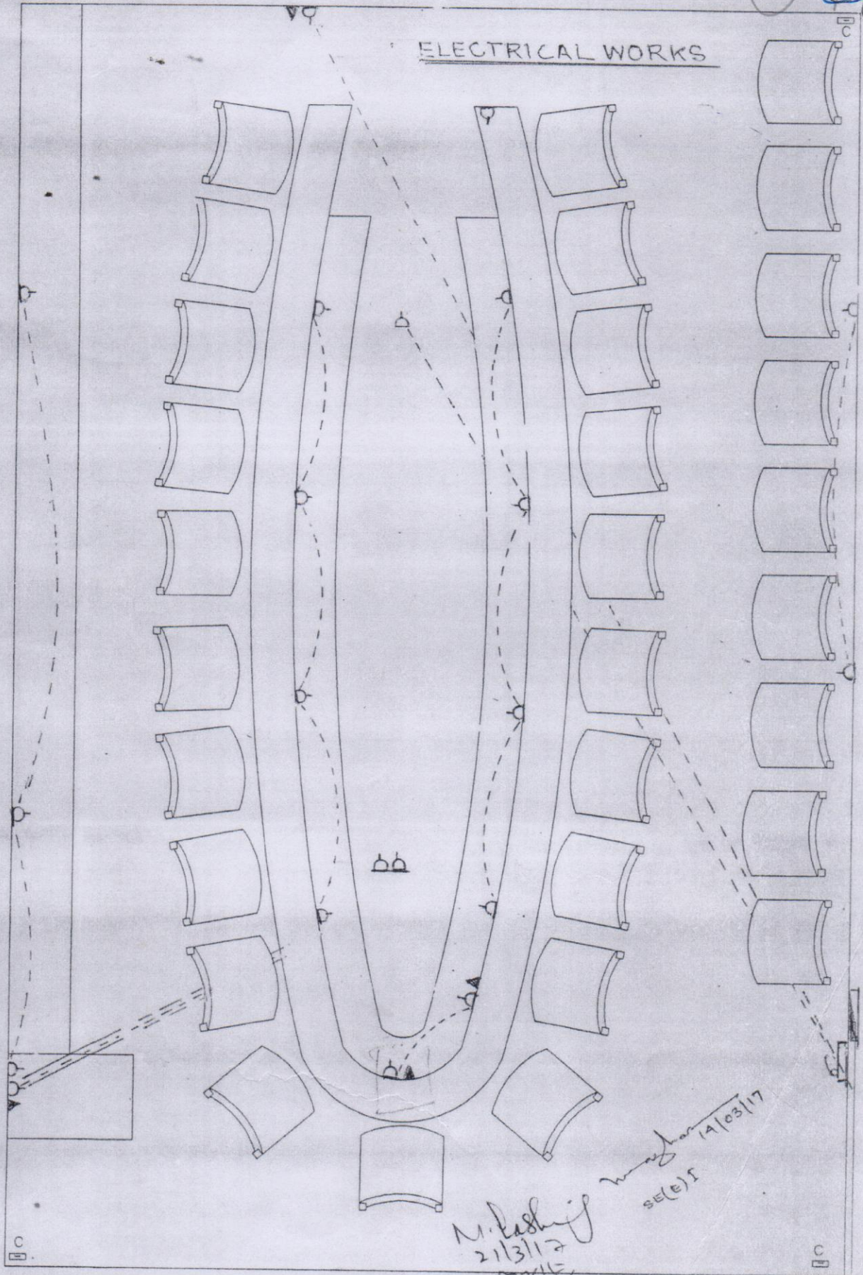
LAYOUT DRAWING OF POWER POINT AND DATA POINT.
