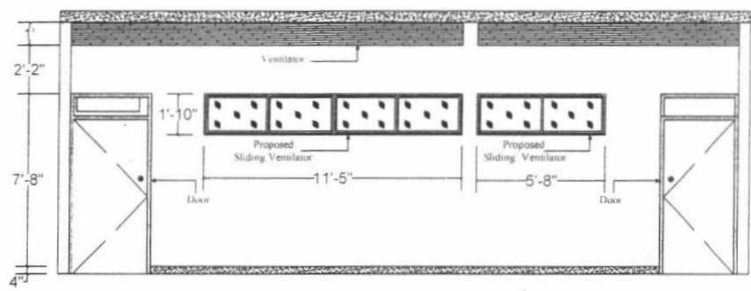
EXISTING ELEVATION-2
