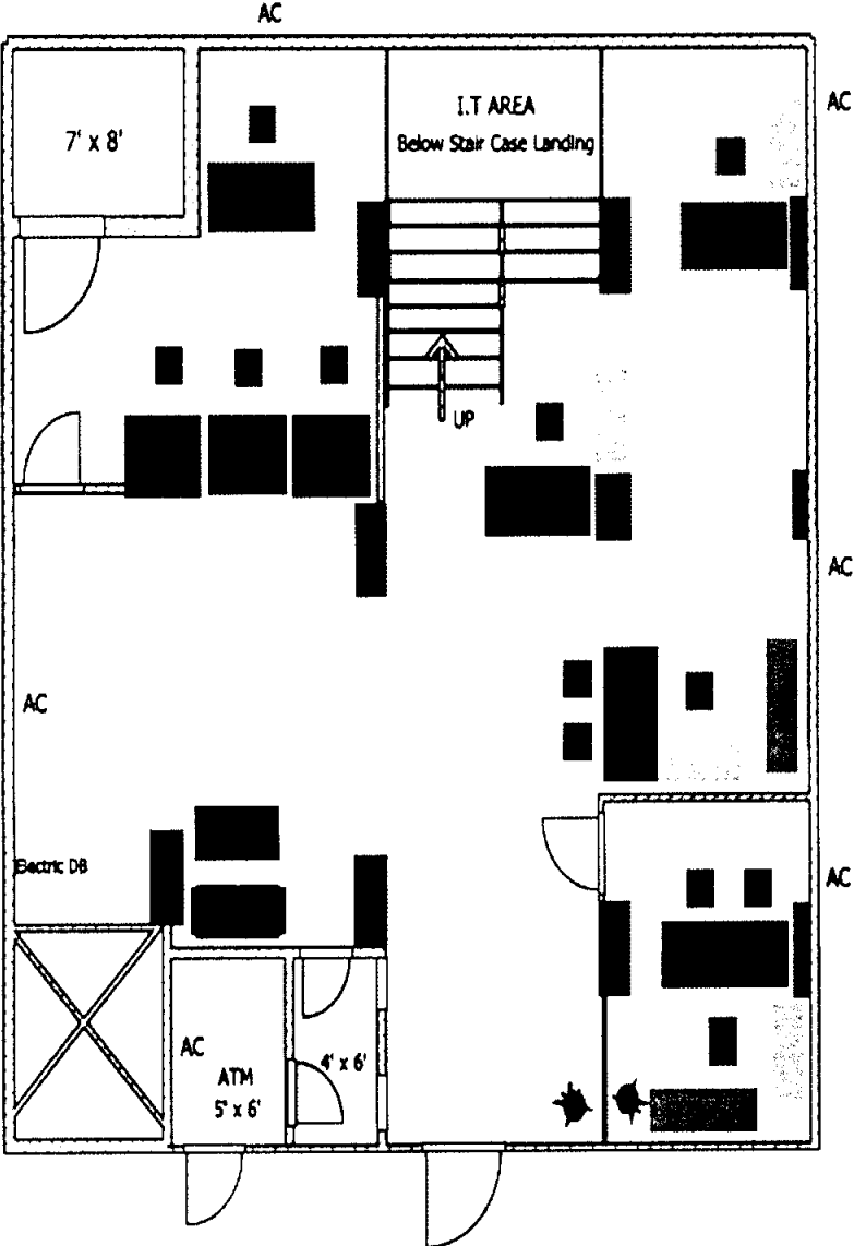
PROPOSED PLAN GROUND FLOOR - RASHID MINHAS ROAD KARACHI BRANCH Area 1400 Sqft
