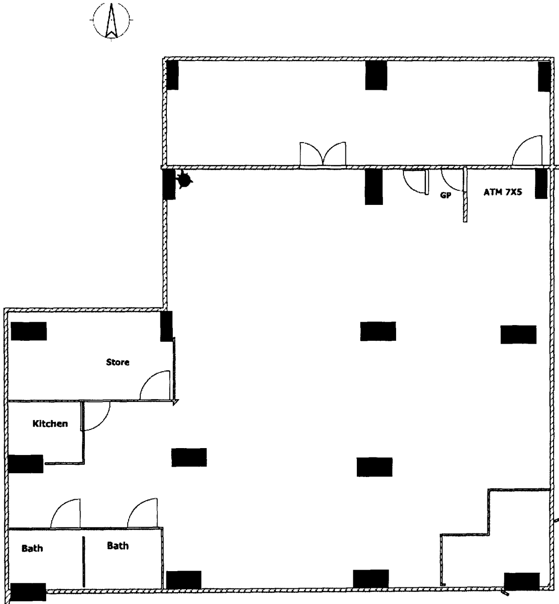
PROPOSED KARIMABAD BRANCH ( Mezzanine )
