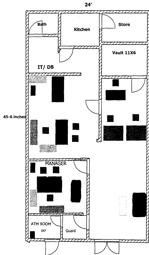
PROPOSED MERAN BRANCH (1100 SFT)
