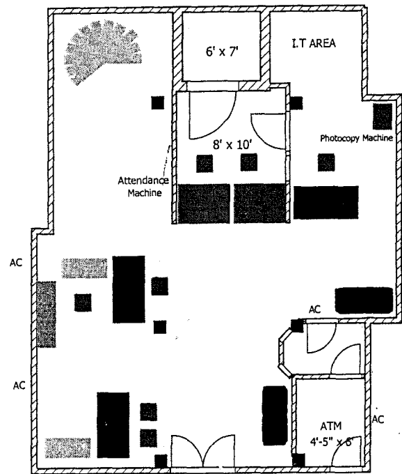
25' PROPOSED PLAN - MARDAN BRANCH GROUND FLOOR Area 860 Sqft Total Area (Ground + First Floor) = 1580 Sqft
