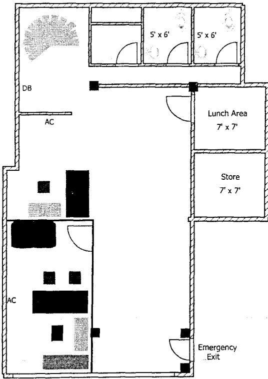
19' PROPOSED PLAN - MARDAN BRANCH FIRST FLOOR Area 724 Sqft
