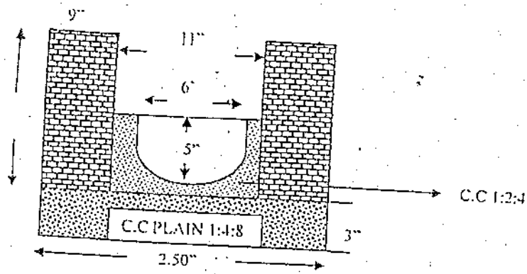
TYPE - I DRAIN
