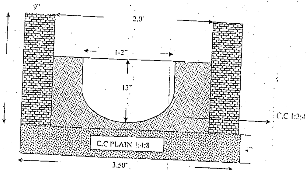
TYPE - III DRAIN
