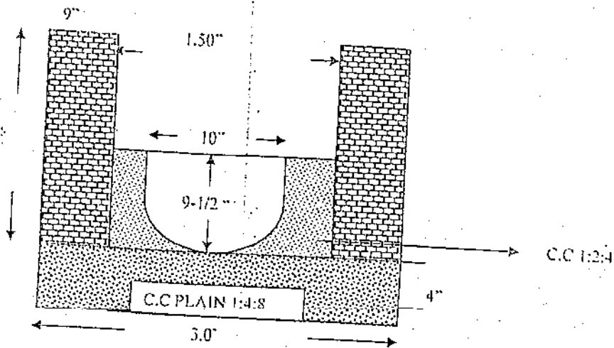
TYPE - II DRAIN
